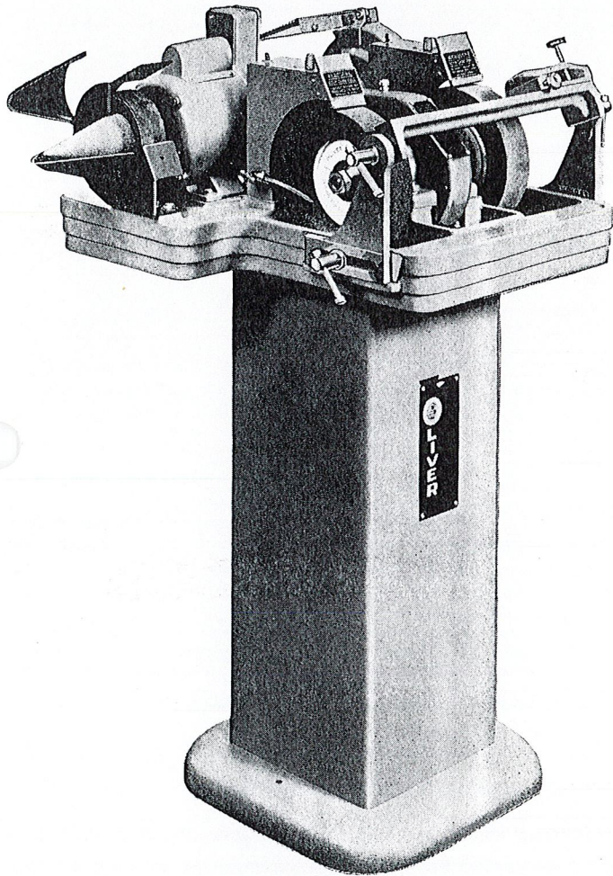
Left side view showing Oilstone wheels, emery cone and stropping wheel.
