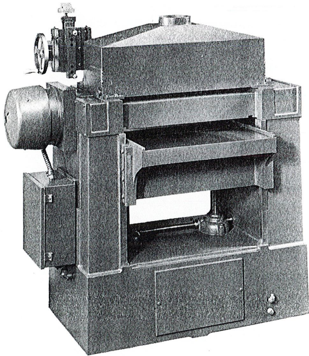
Rear view of 299 Surfacer with dust hood attached.
