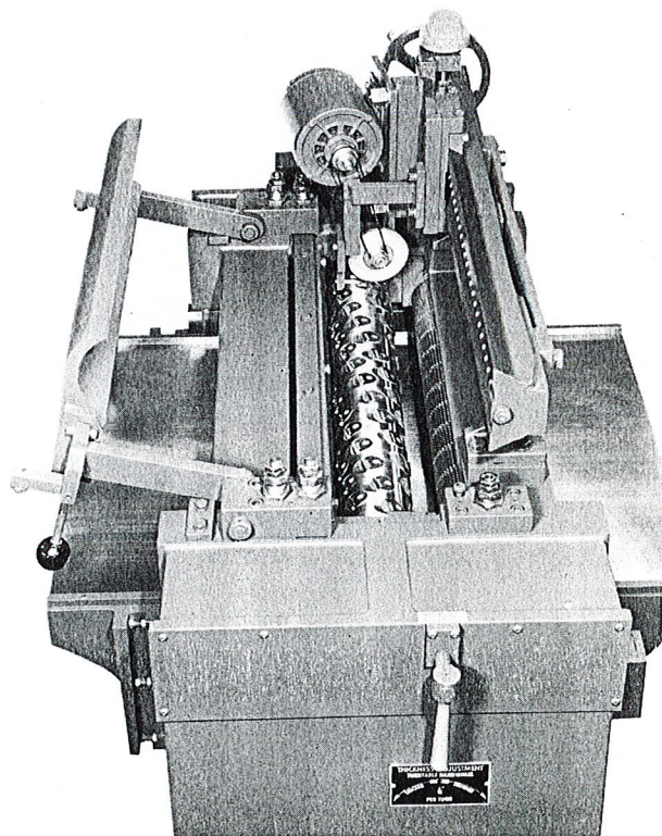
View showing the patented Inserted Tooth Carbide Bit Cutter head mounted in the machine with the Knife Grinding Attachment in grinding position.
