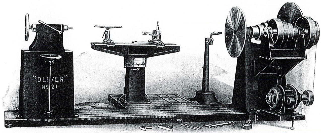
“OLIVER” NO. 21-AC PATTERN MAKERS’ COMBINATION LATHE Rear View showing ease with which Tail Stock Column and Carriage Stand can be moved to any place desired. Note — Rest Holder shown on left end of Carriage is not regular equipment.
