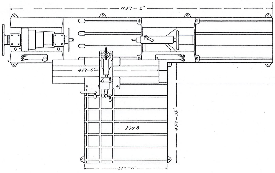
Etching showing Floor Plan of Machine with Tail Stock and Extension Sole Plate.
