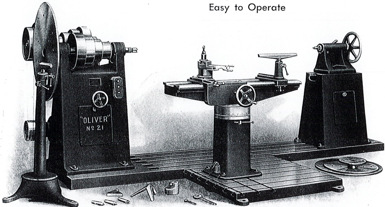
No. 21-AC "OLIVER" COMBINATION PATTERN LATHE. View Showing Tail Stock and Extension Sole Plate. Extended Sole Plate for increased capacity either for lengths or to facilitate the use of tool post around pit on outside face plate at additional cost. Note—Rest Holder shown on right end of carriage is not regular equipment.
